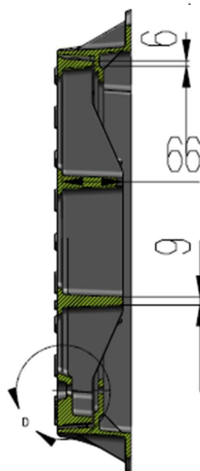
SECTION C-C
