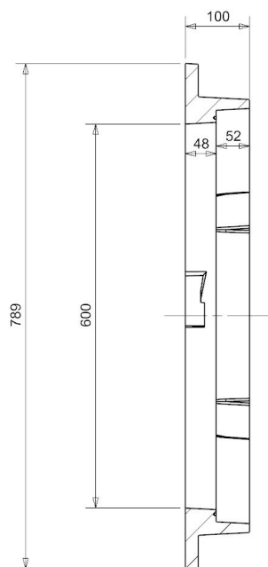
SECTION C-C
